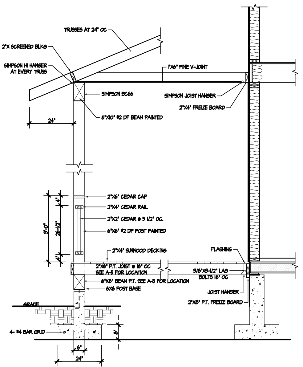
SECTION DETAIL AT PORCH SCALE: 3/4" = 1'-0"
