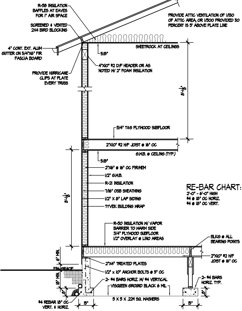
TYPICAL FRAMING DETAIL SCALE: 1/2" = 1'-0"
