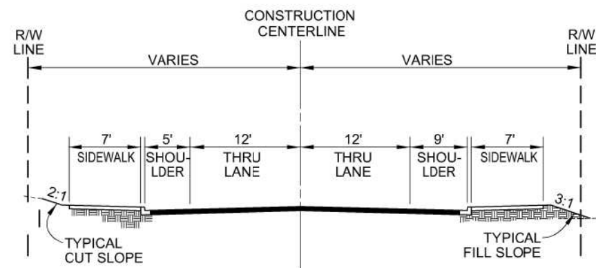
TYPICAL ROADWAY CROSS SECTION
