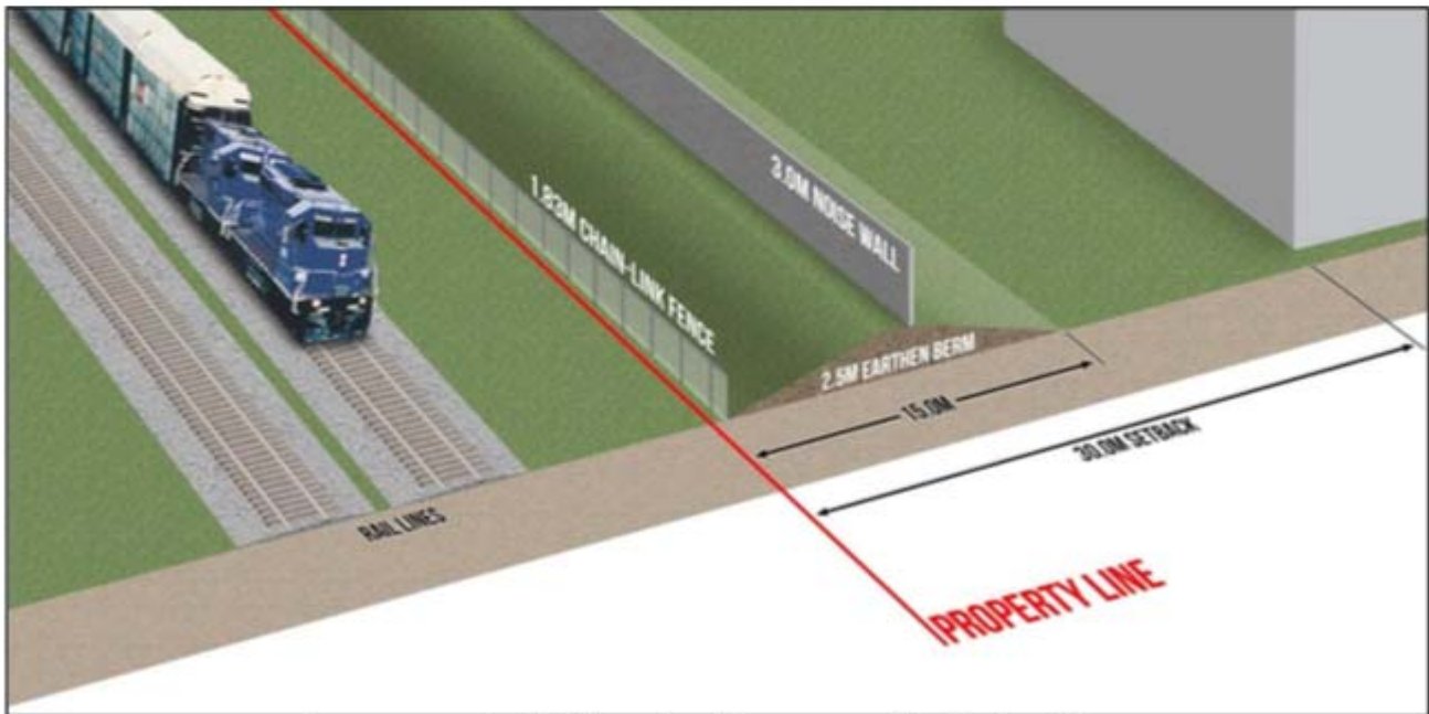
Recommended Mitigation Measures: Bird's Eye View
