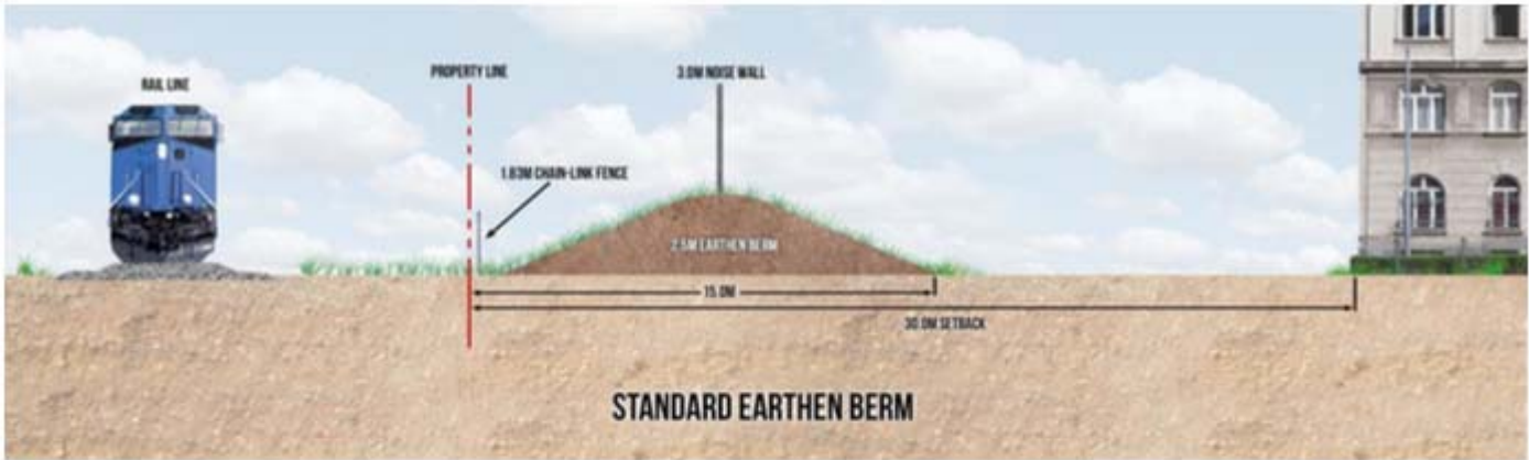
Recommended Mitigation Measures: Cross-Section
