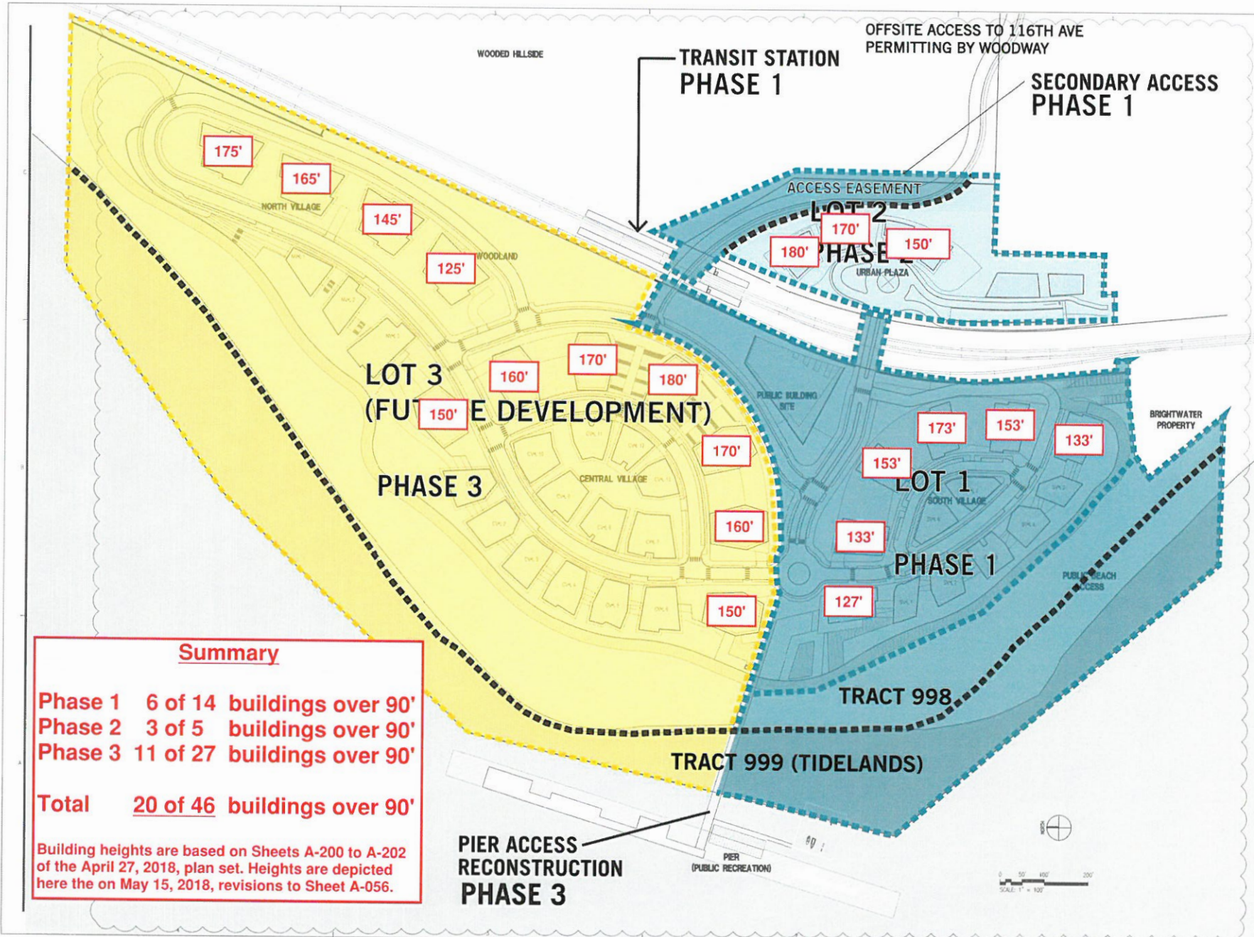
P-3 Phasing Plan Sheet 1 A-056 - depicted from May 15, 2018 revision PFN: 11 101457 LU
